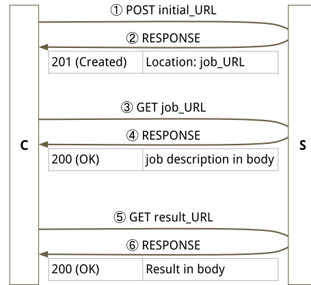
Figure 5: Asynchronous protocol
