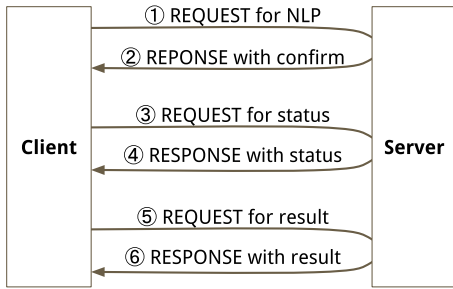
Figure 3: General asynchronous protocol with status checking
